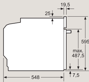
HB479G5A7F / HB478G5B7 / HB479G0A3 / HR478G5B7F / HB472G0B3 / HR472G0B3
