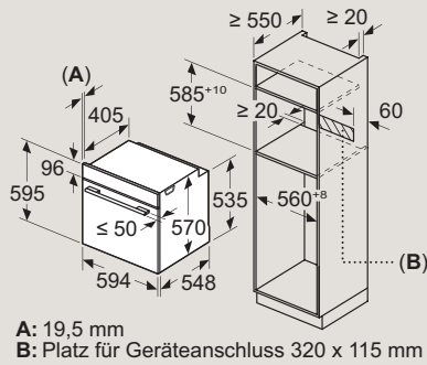
HB479G5A7F / HB478G5B7 / HB479G0A3 / HR478G5B7F / HB472G0B3 / HR472G0B3
